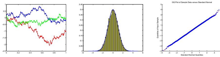
FIGURE 1. Left: Sample paths for standard Brownian motion; Center: histogram of W(1) vs. the pdf of the standard normal; Right: quantile-quantile plot of W(1) .
