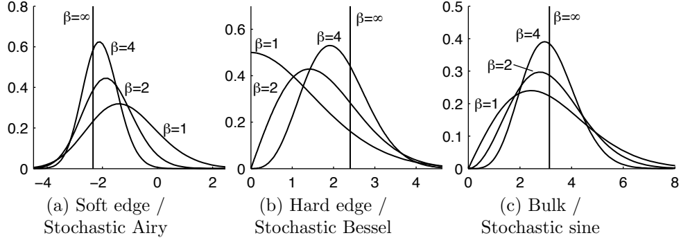
FIGURE 2. Local eigenvalue behavior
