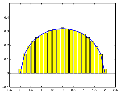
(a) Semicircle Law
