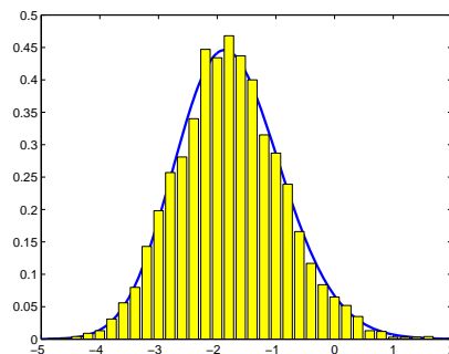
(b) Tracy-Widom distribution
