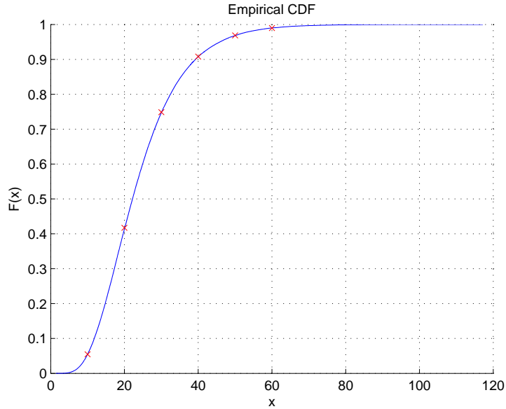
FIGURE 3. The empirical (blue) and analytic (red) cdf's of the largest eigenvalue of the general \beta -Wishart Ensemble.
